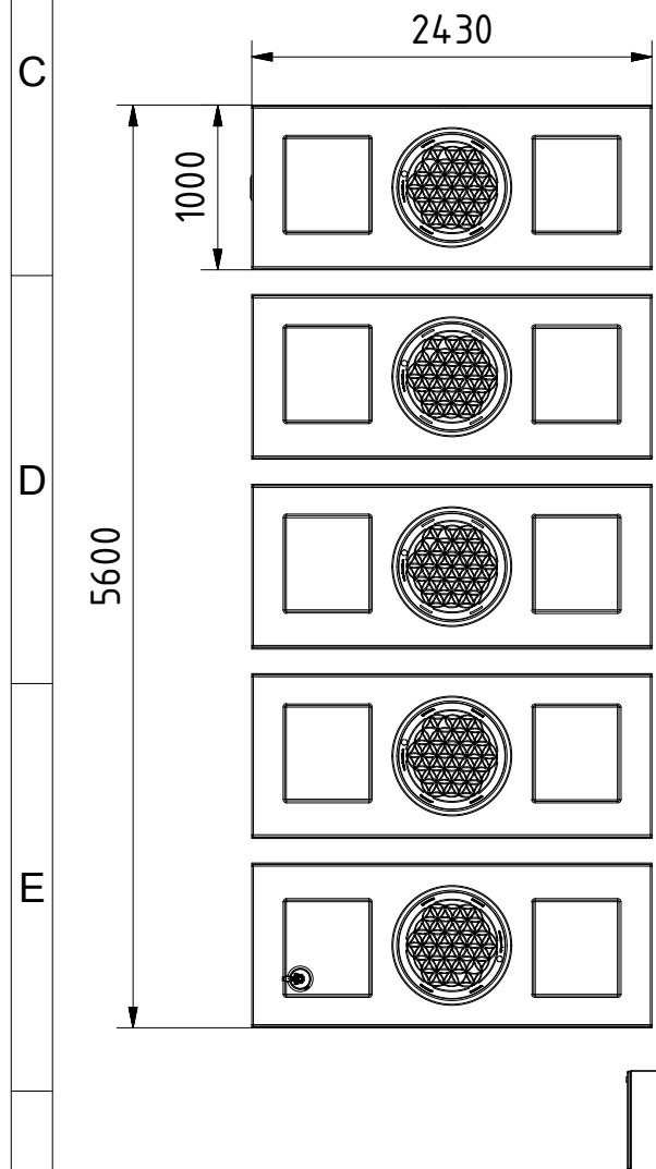
sedimentation tank Sedimentationstank 1 x 4000 l
