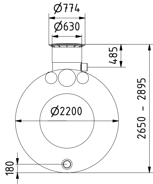
retention throttle DN 150 Retentionsdrossel
